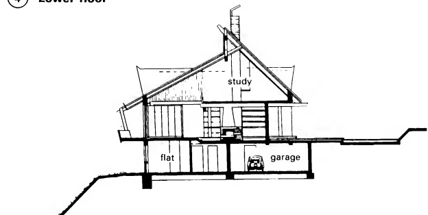
⑥ Section
